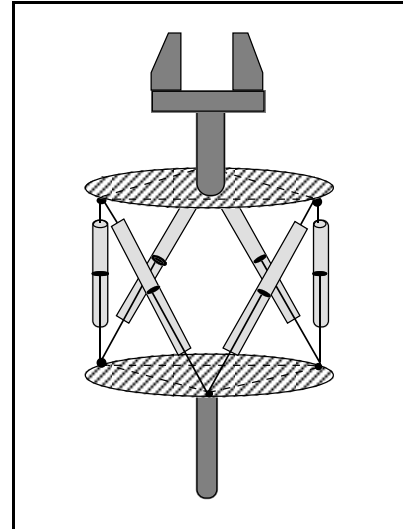
Fig. 2. A six DOF Stewart platform type robotic wrist.
