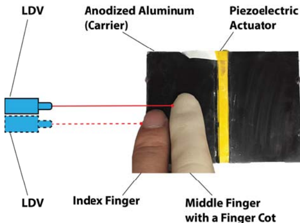
Fig. 1. Top view of the setup in Experiment 1.
