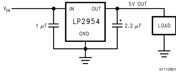
5V Regulator
