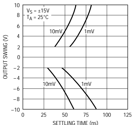
LT1220 • TPC11
