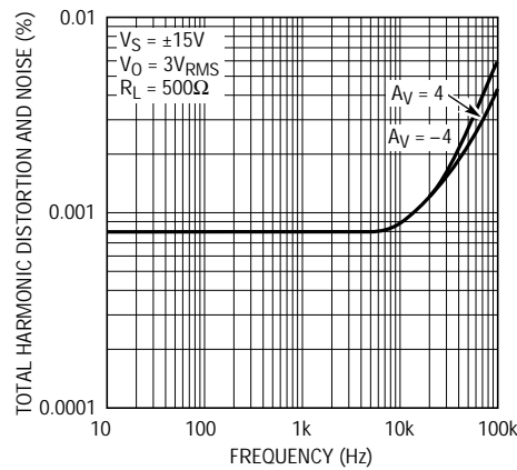
LT1220 • TPC18
