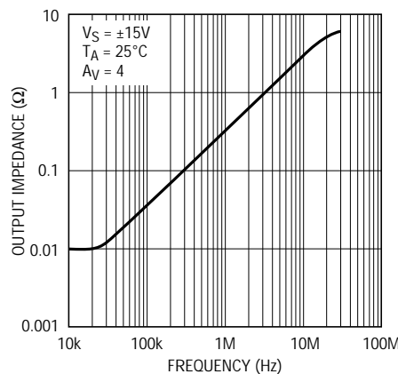
LT1221 • TPC15
