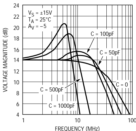
LT1221 • TPC14
