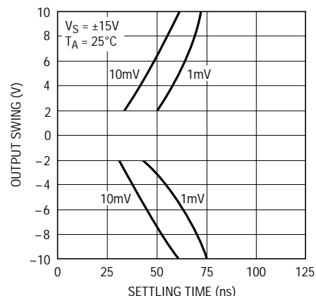
LT1221 • TPC12
