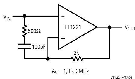
Lag Compensation
