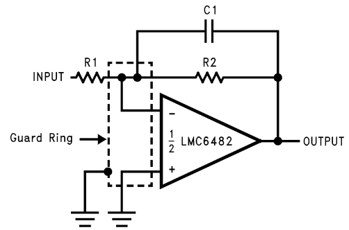
Inverting Amplifier
