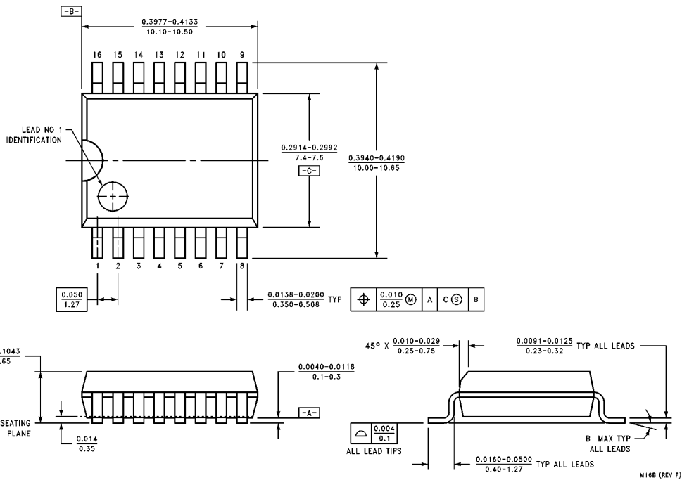
16-Lead Small Outline Package (WM) Order Number LM613IWM NS Package Number M16B
