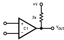
FIGURE 16. Basic Comparator
