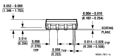
8-Lead (0.150" Wide) Molded Small Outline Package, JEDEC Order Number LM6132AIM, LM6132BIM, LM6132AIMX or LM6132BIMX NS Package Number M08A
