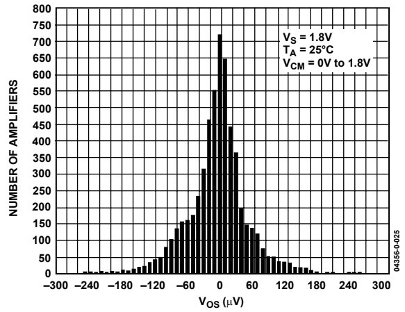
Figure 28. V_{OS} Distribution
