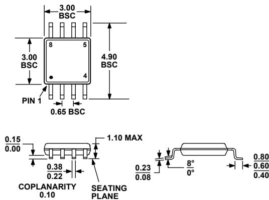
Figure 50. 8-Lead MSOP Package (RM-8) Dimensions in millimeters
