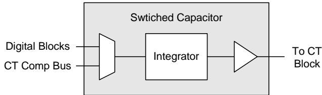
Figure 24-11. Analog Switch Capacitor PSoC Block for the CY8C21x34, CY8C21x23, CY7C603xx, and CYWUSB6953 PSoC Devices
