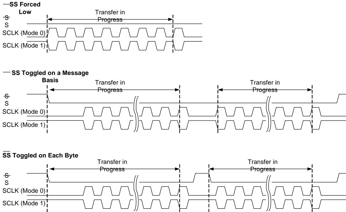
Figure 17-18. SPI Status Timing for Modes 0 and 1
