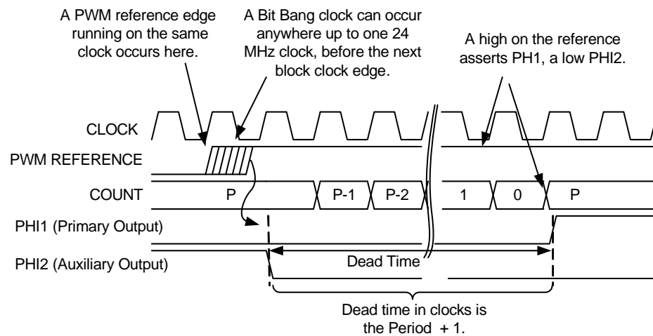
Figure 17-9. Basic Dead Band Timing
