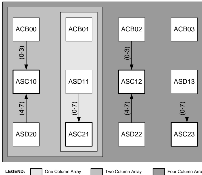
Figure 19-6. CMux Connections
