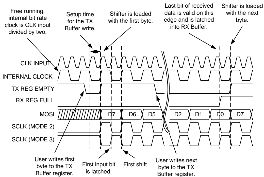
Figure 17-17. Typical SPI Timing in Mode 2 and 3
