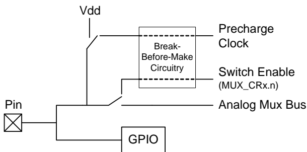
Figure 33-2. IO Pin configuration for the CY8C21x34, CY7C603xx, and CYWUSB6953
