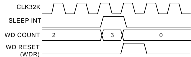
Figure 12-4. Watchdog Reset
