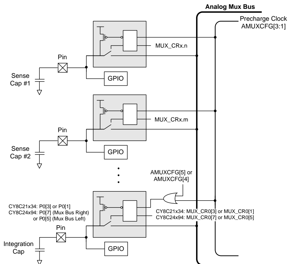
Figure 33-3. CY8C24x94, CY8C21x34, CY7C64215, CY7C603xx, CYWUSB6953 Capacitance Sense Example Diagram
