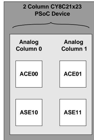
Figure 24-4. Array of Analog PSoC Blocks for the CY8C21x34, CY8C21x23, CY7C603xx, and CYWUSB6953 PSoC Devices
