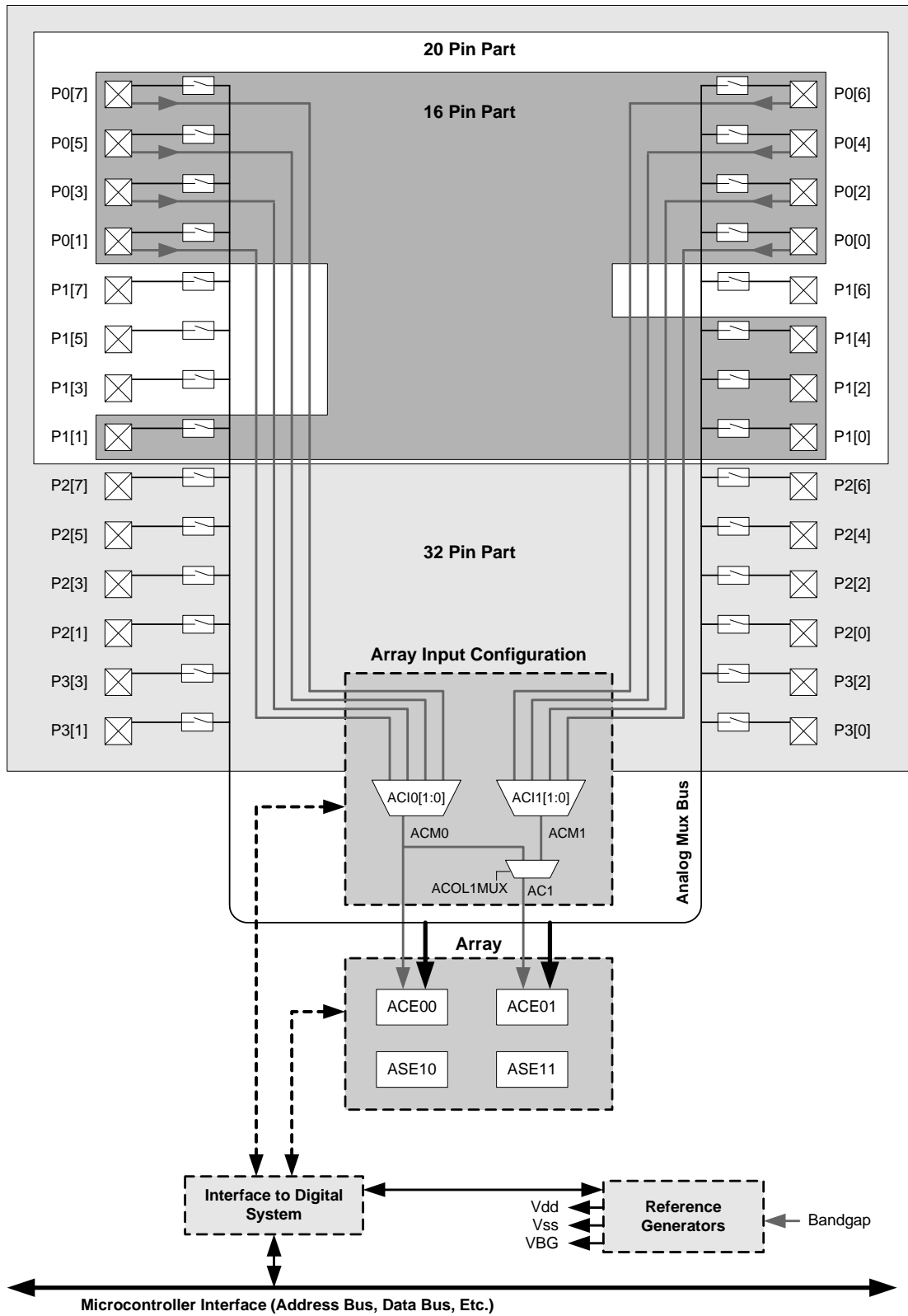
Figure 24-8. Two Column Limited Analog Pin Block Diagram for the CY8C21x34, CY7C603xx, and CYWUSB6953
