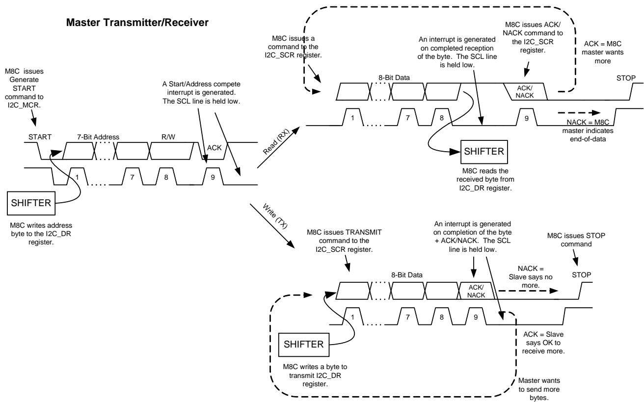
Figure 28-3. Master Operation
