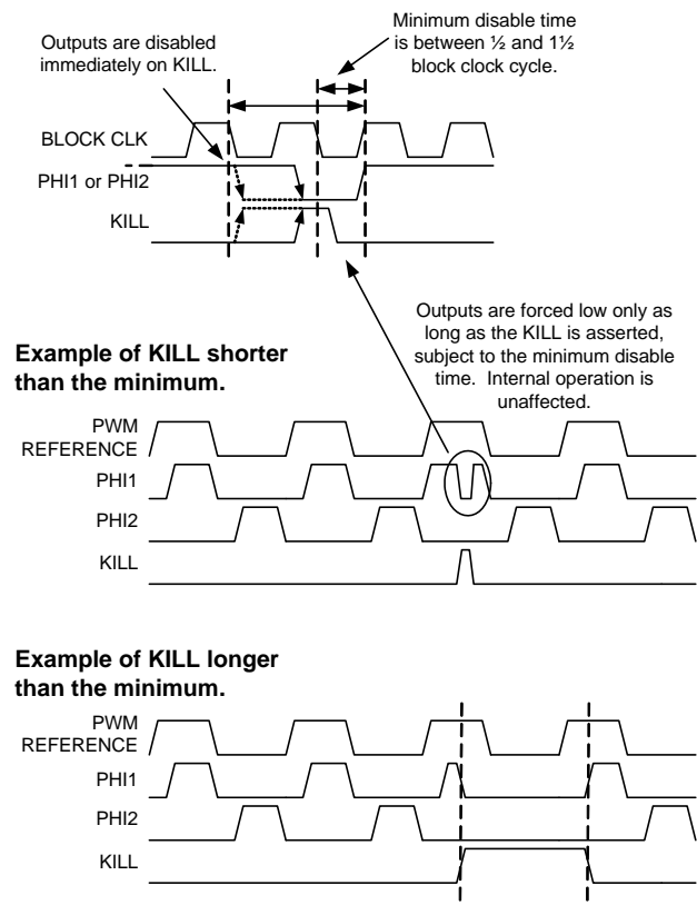
Figure 17-14. Asynchronous Restart Kill Mode
