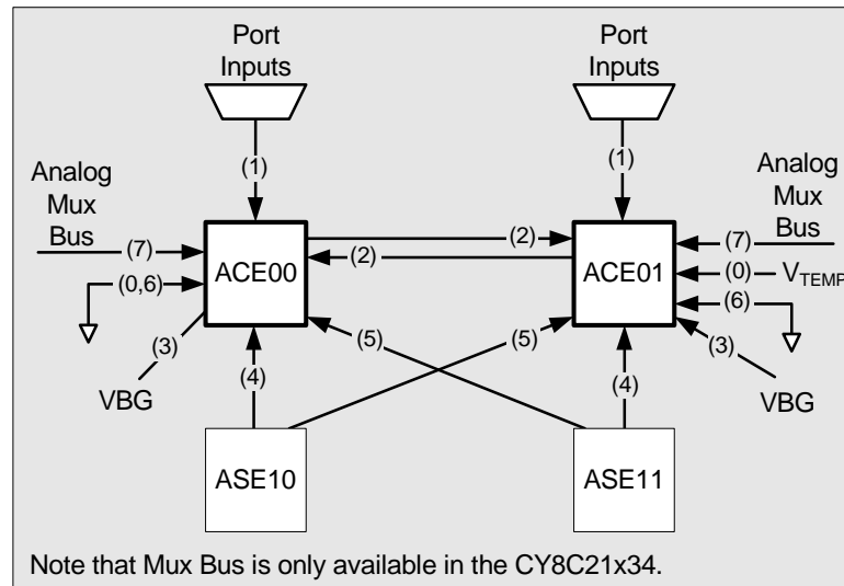
Figure 24-6. PMux Connections for the CY8C21x34, CY8C21x23, CY7C603xx, and CYWUSB6953 PSoC Devices
