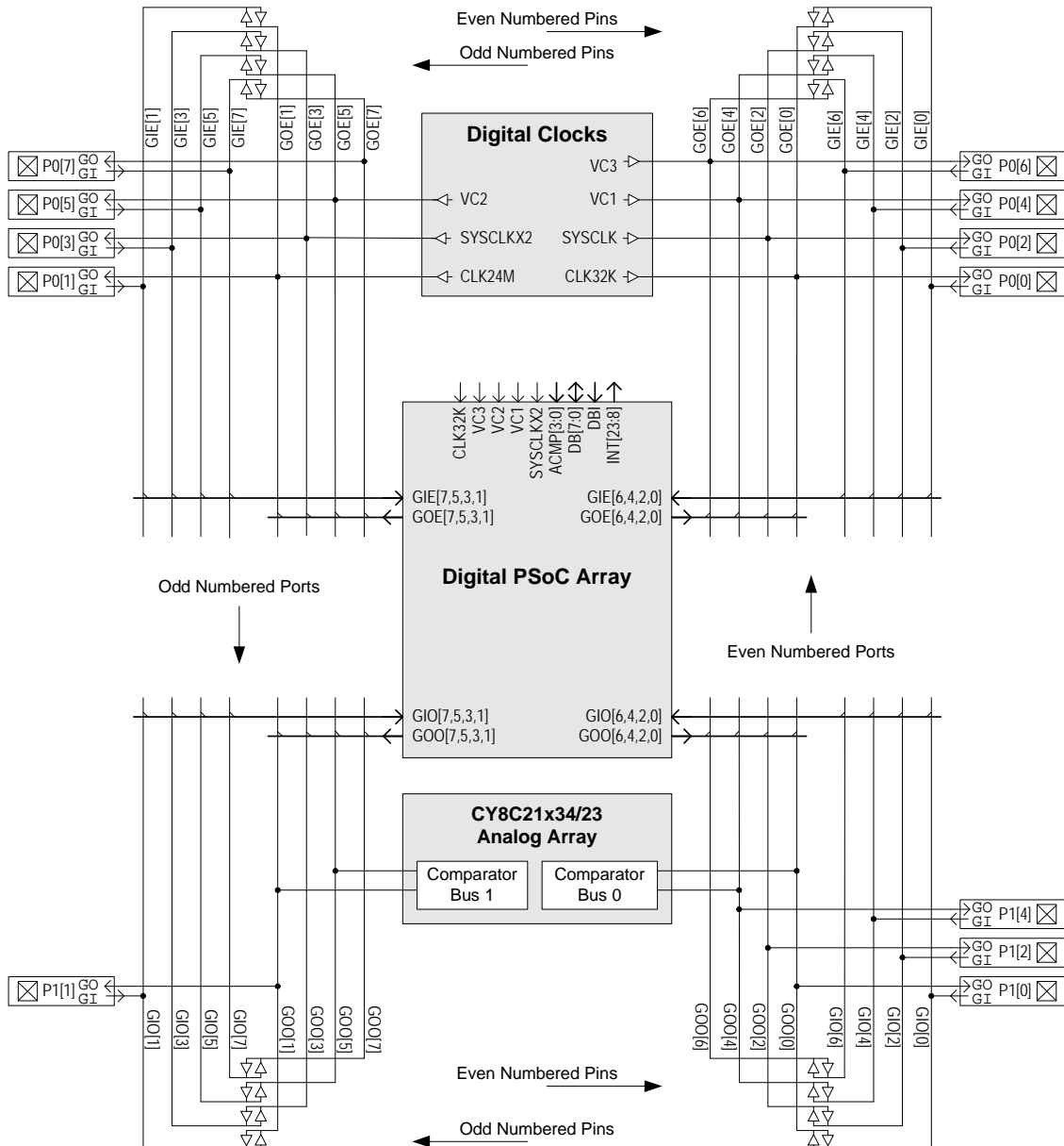
Figure 14-2. Global Interconnect Block Diagram for the CY8C21x34/23, CY7C603xx, and CYWUSB6953 16-Pin Package
