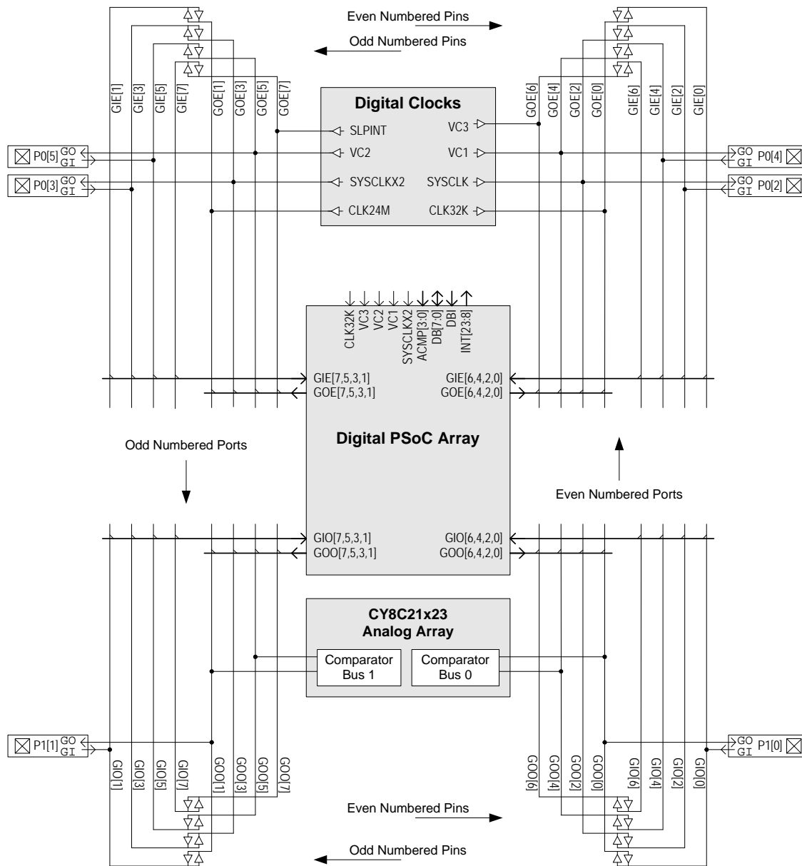
Figure 14-1. Global Interconnect Block Diagram for an 8-Pin Package
