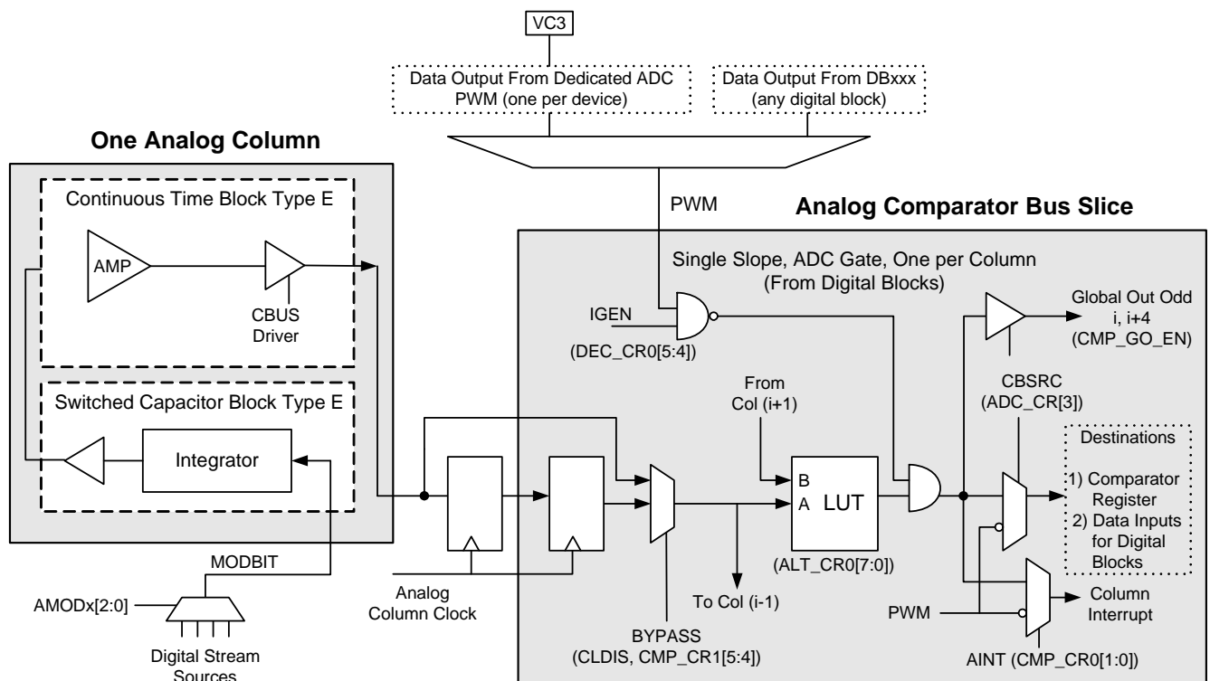
Figure 24-1. Analog Comparator Bus Slice of the CY8C21x34, CY8C21x23, CY7C603xx, and CYWUSB6953 PSoC Devices
