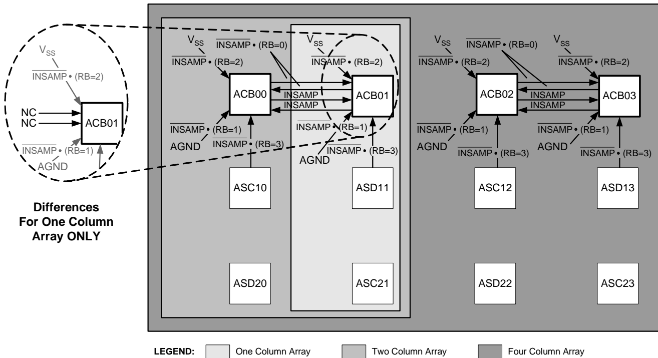
Figure 19-4. RBotMux Connections
