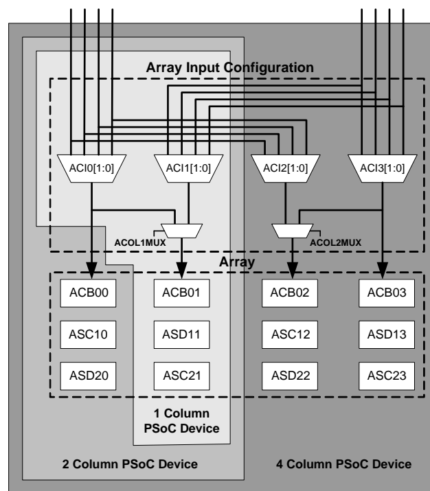
Figure 20-1. Analog Input Configuration Column Overview
