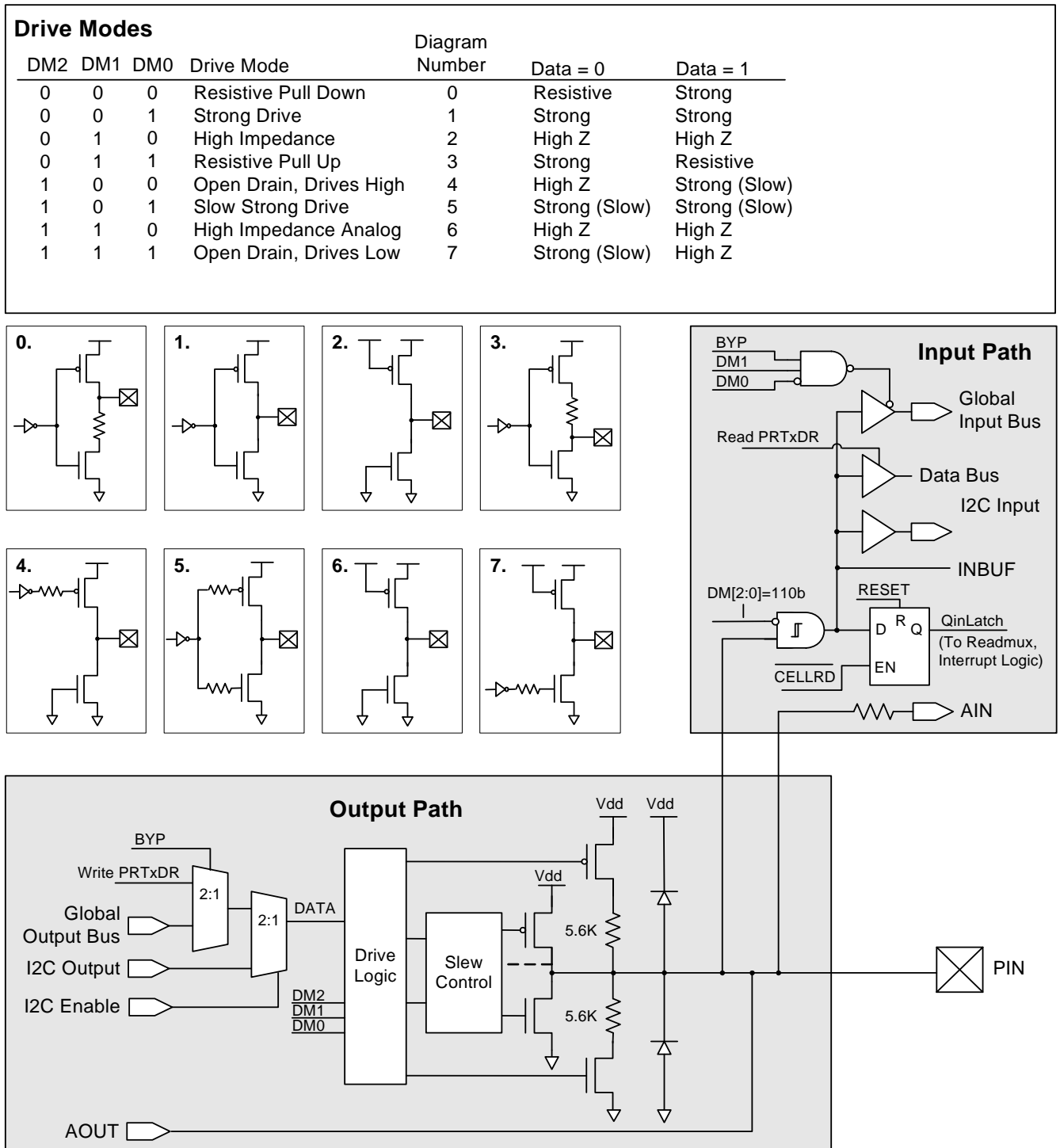
Figure 6-1. GPIO Block Diagram
