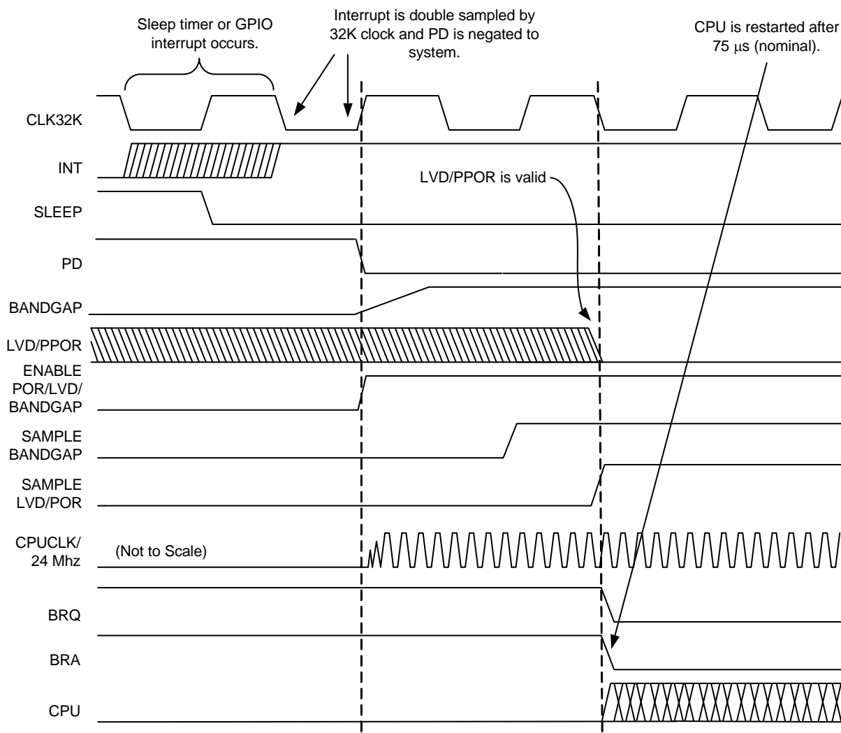
Figure 12-2. Wakeup Sequence
