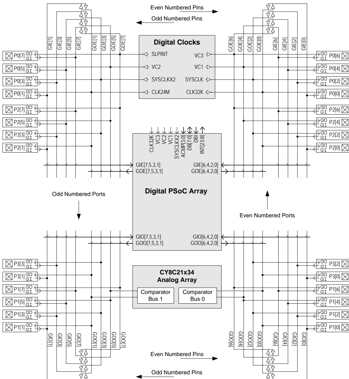
Figure 14-5. Global Interconnect Block Diagram for CY8C21x34, CY7C603xx, and CYWUSB6953 32-Pin Packages
