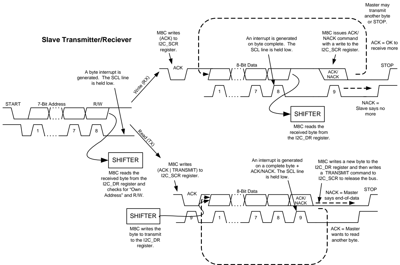
Figure 28-2. Slave Operation
