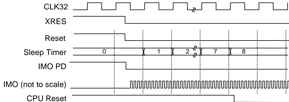
Figure 30-4. Key Signals During POR and XRES
