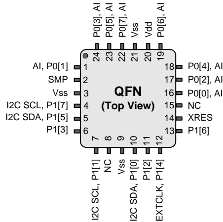
CY8C21323 PSoC Device
