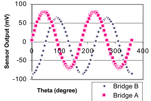
HMC1512 output voltage vs. magnetic field angle
