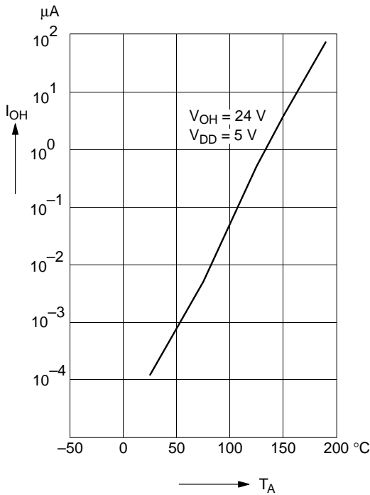
Fig. 15: Typical output leakage current versus temperature
