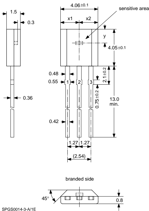
Fig. 3-1: Plastic Transistor Single Outline Package (TO-92UT)
