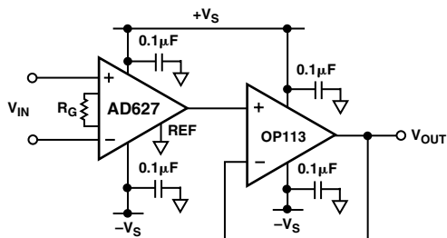
Figure 7. Output Buffering
